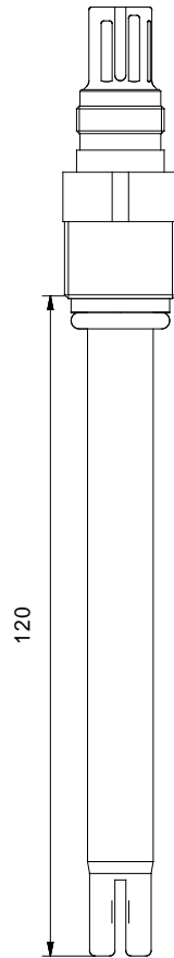
LTG1/22VP Dimension in mm
